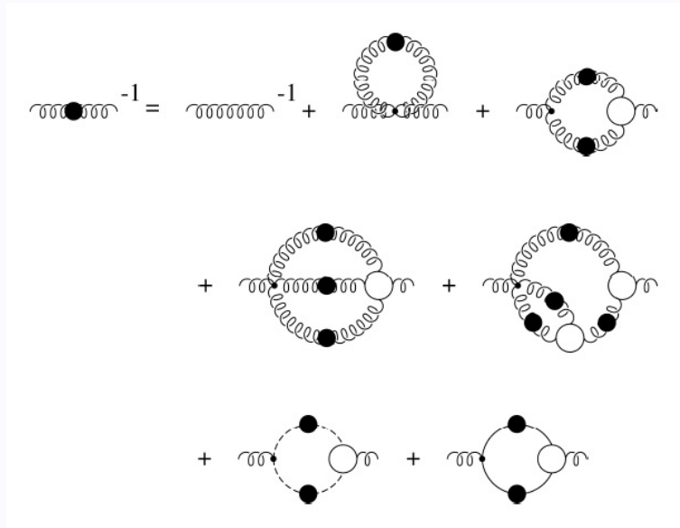
DSE for gluon propagator
