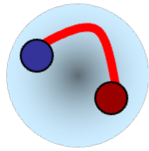
Hybrid
