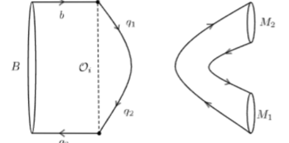
(h) CPA: Connected Penguin-Annihilation
