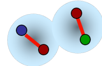
Hadronic molecule
