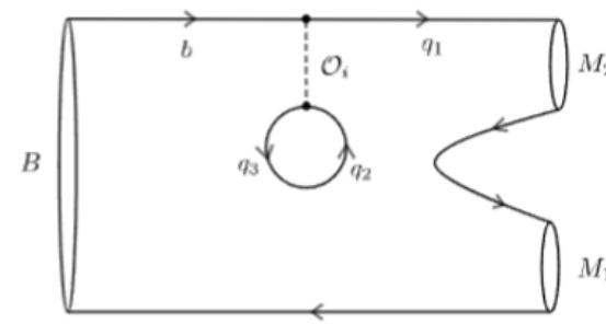
(c) DP: Disconnected Penguin
