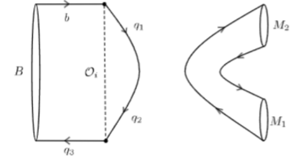
(h) CPA: Connected Penguin-Annihilation
